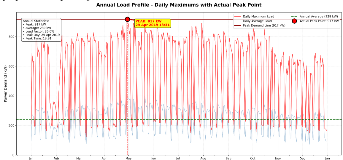
Figure 4. Daily cooling load profile demonstrating peak requirements and baseline load.
