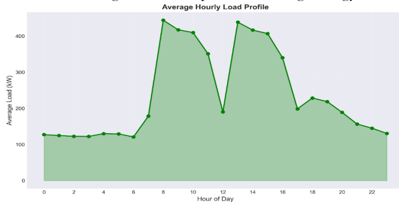
Figure 7. Average hourly load profile revealing occupancy-driven morning ramp-ups.
