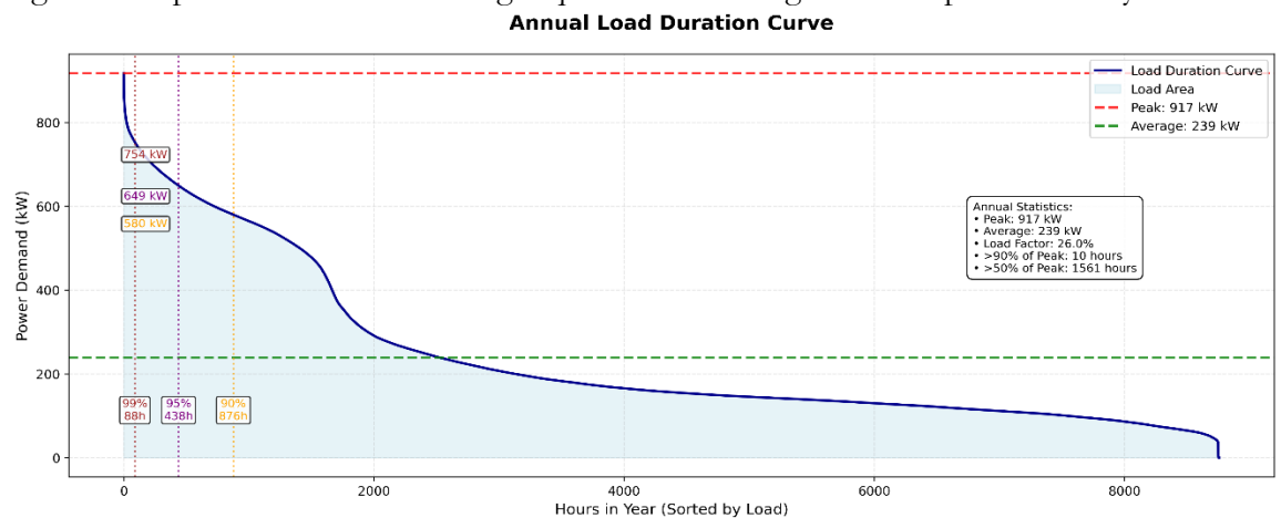
Figure 5. Annual load duration curve confirming non-simultaneous peak loads.
