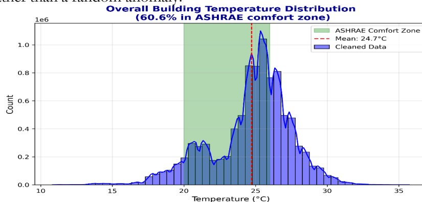
Figure 13. Thermal comfort compliance against ASHRAE 55 limits.
