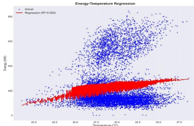
Figure 12. Energy–Temperature regression ( R^2 = 0.023 ), confirming internal gains.
