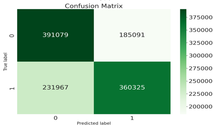
Figure 17. Confusion matrix for Decision Tree (without timestamp). Test accuracy: 92%.
