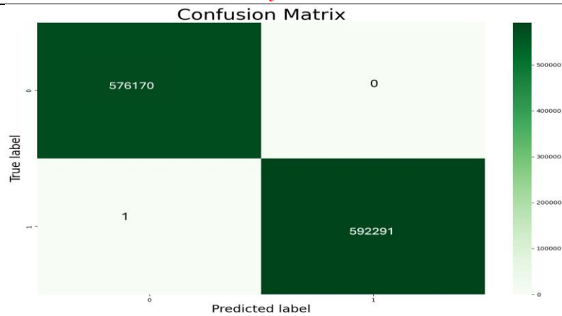
Figure 15. Confusion matrix for ANN (with timestamp). Test accuracy: 100%.
