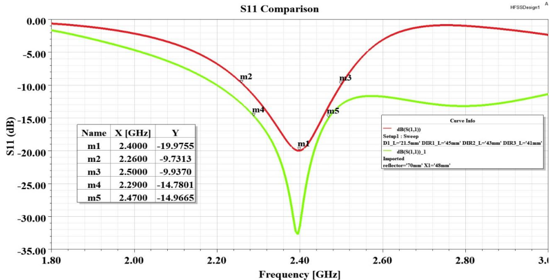
Figure 4. Comparison between Yagi Uda and Corner Reflector Antenna showing return loss for both antennas at 2.4GHz
