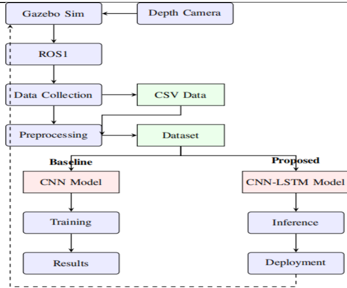
Figure 3. Flow Chart of Model Architecture
