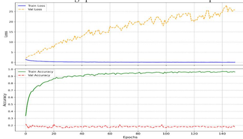
Figure 4. CNN-Only Model Performance
