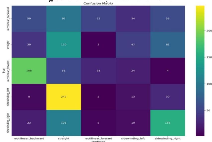
Figure 5. CNN-Only Model Performance
