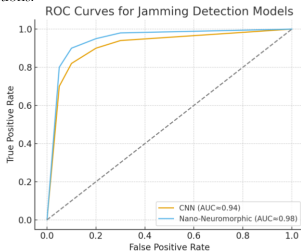
Figure 6. ROC Curves for Jamming Detection Models
