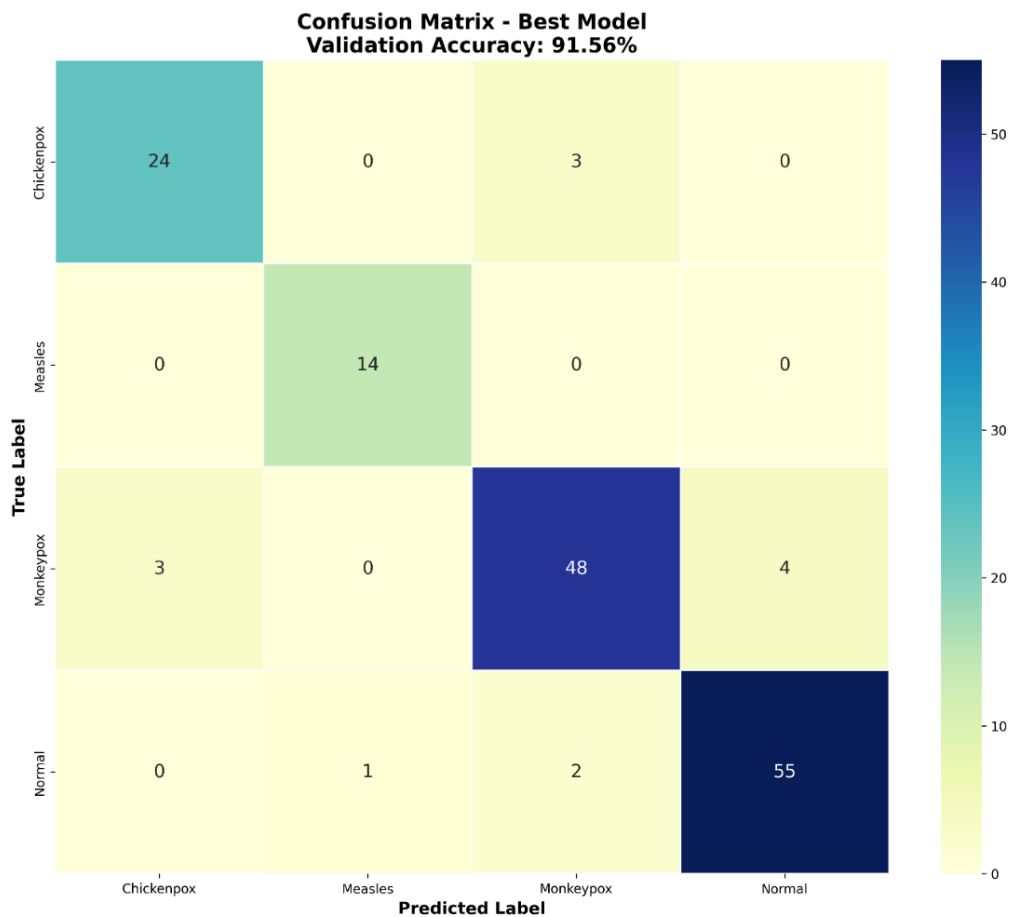
Figure 4. Confusion Matrix
