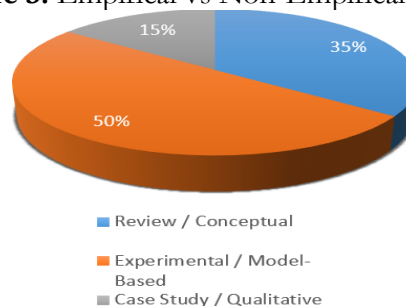
Figure 4. Methodology Classification
