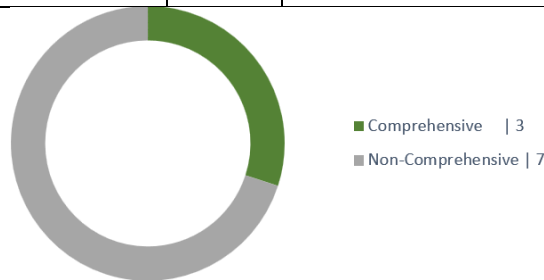
Figure 8. Completeness Score
