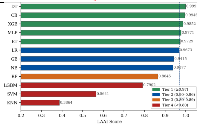
Figure 6. LAAI-Ranked Model Performance.
