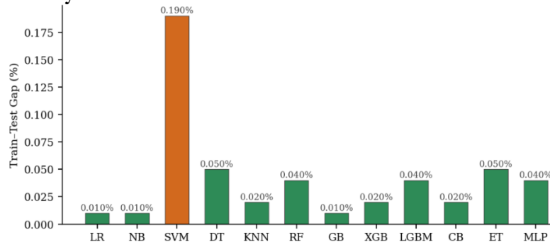
Figure 8. Generalization Gap ( | \text{Train Accuracy} - \text{Test Accuracy} | ).
