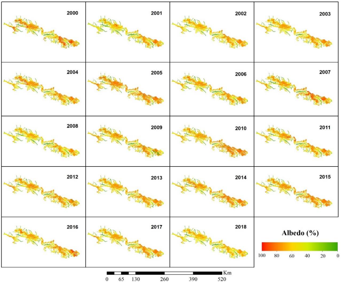
Figure 4. MODIS-observed surface albedo of the Karakoram glaciers from 2000 to 2018
