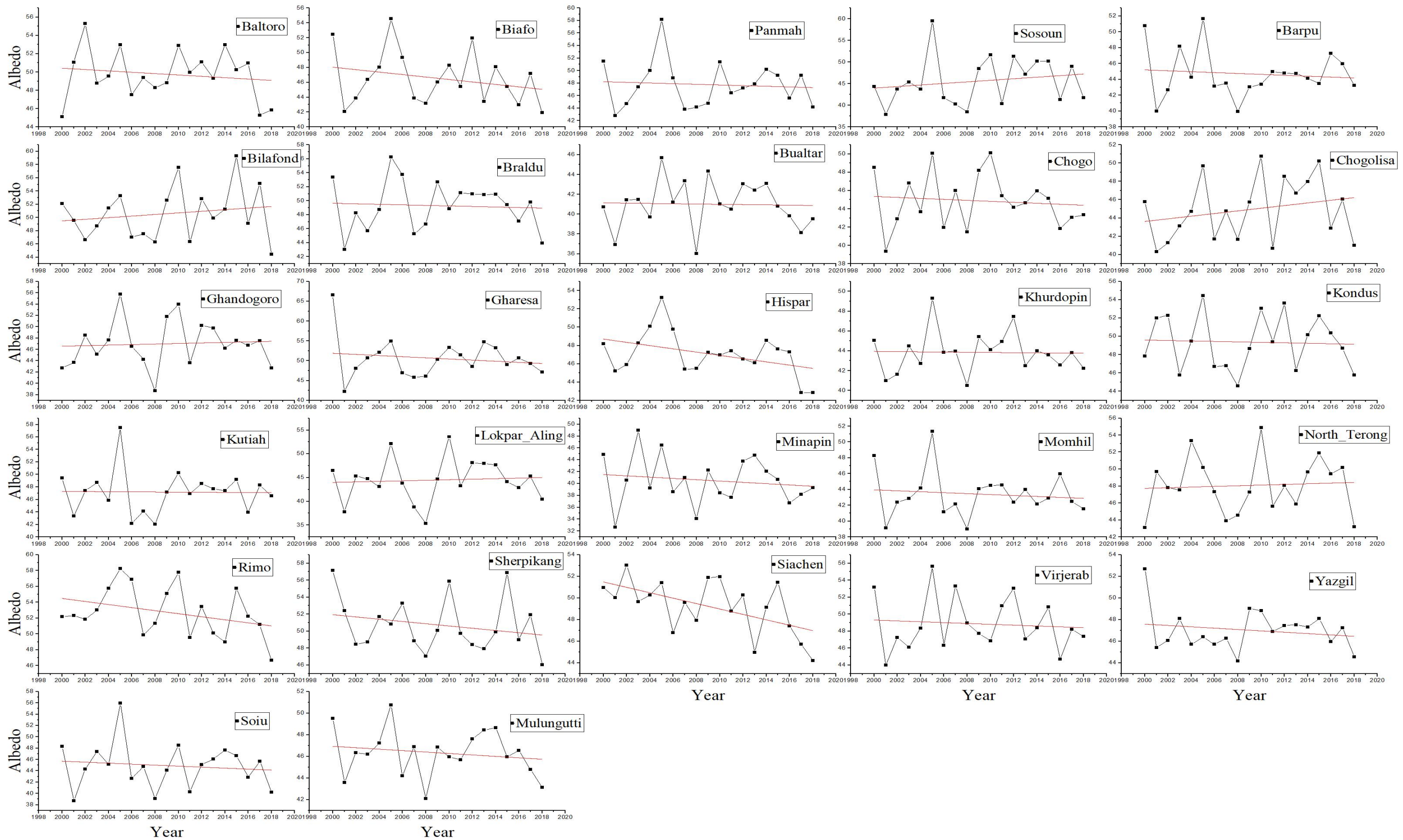
Figure 7. Graph showing trend of the variation in summer albedo for the glacier under the study from 2000 to 2018
