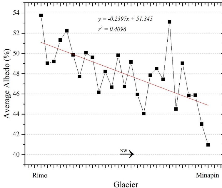
Figure 8. The direction of the decrease in albedo showing that the albedo is decreasing towards the north-western part of the Karakoram
