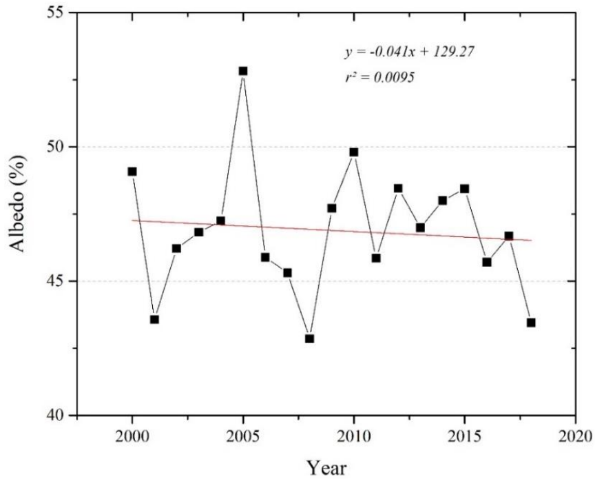
Figure 5. Surface albedo variation in Karakoram glaciers during the summer seasons of 2000 to 2018. The red line shows the trend of decreasing surface glacier albedo
