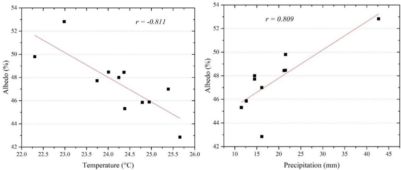
Figure 12. Correlation of surface albedo with temperature and precipitation. Albedo have a significant negative and significant positive correlation with temperature and precipitation respectively.
