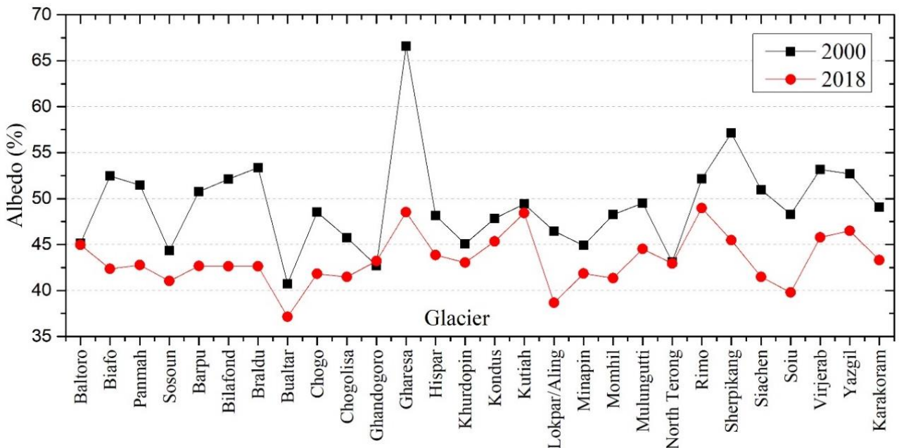
Figure 10. Graph showing albedo variation between the year 2000 and 2018. Black graph represents the albedo in year 2000 and red graph represent the albedo in year 2018.
