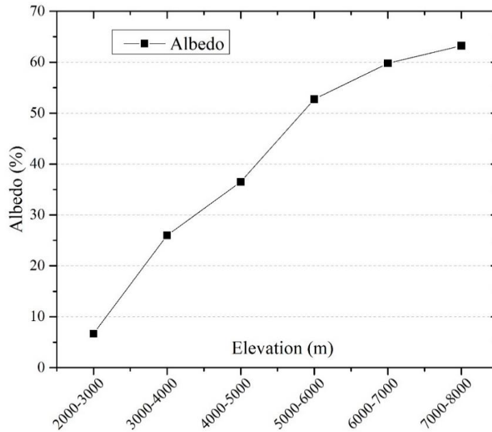
Figure 11. The amount of albedo increases with increasing elevation and as the temperature decreases, causing less glacial melt, which alternately increases the albedo moving towards areas with higher elevations.
