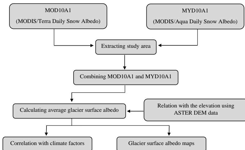
Figure 2. Flow chart of the methodology used for extracting and processing the MODIS albedo data to measure the change in the glacier surface albedo
