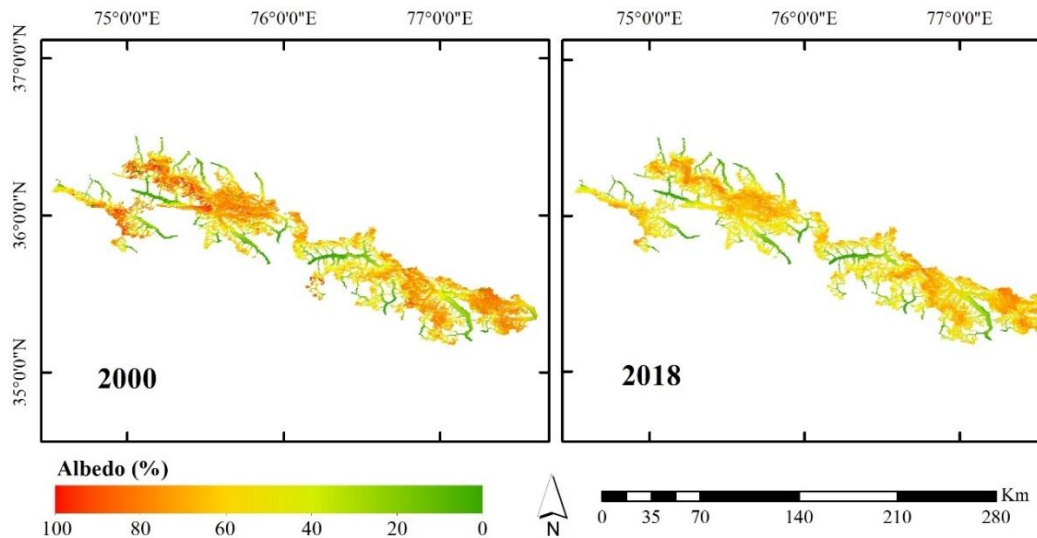
Figure 9. Albedo variation between year 2000 and 2018
