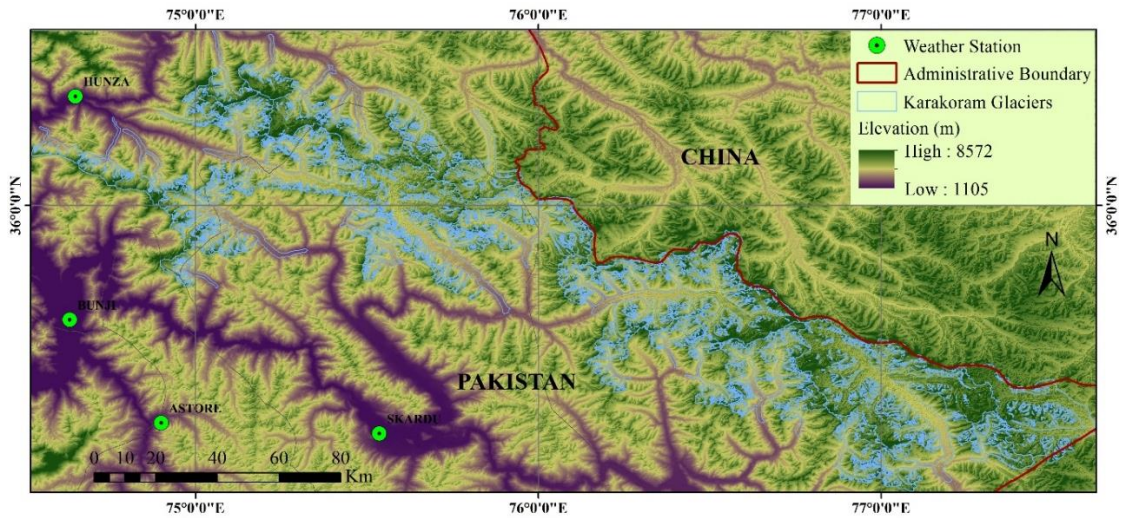
Figure 1. Map of the study area showing the elevation in metres and the Karakoram region under study area highlighted with the light blue colour.
