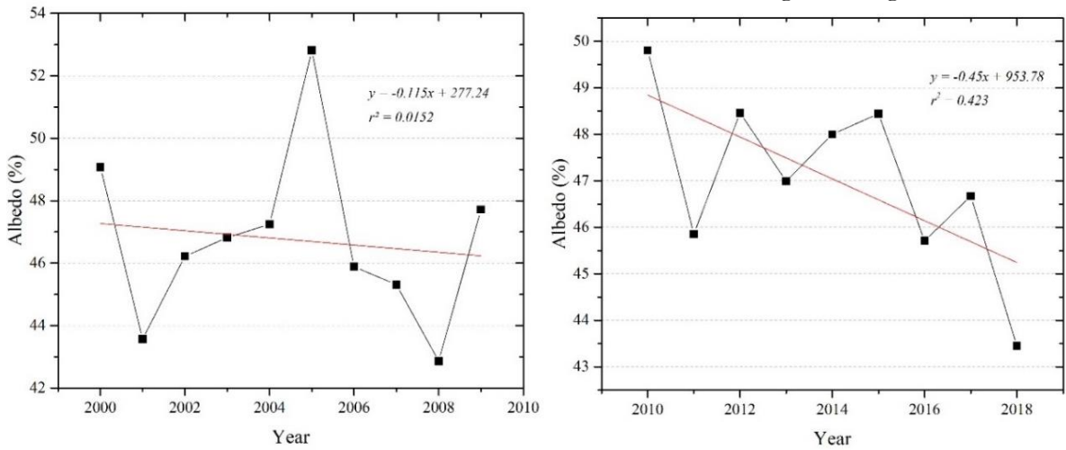
Figure 6. Average snow albedo variations over the past two decades show that the rate of change in albedo is nominal from 2000-2009 compared to 2010-2018.
