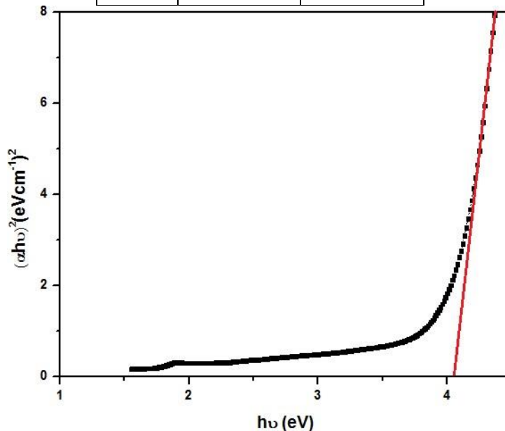
Figure 4: the band gap of NiO/ZnO.
