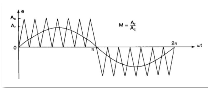
Figure 2. Modulation technique for SPWM pulses.
