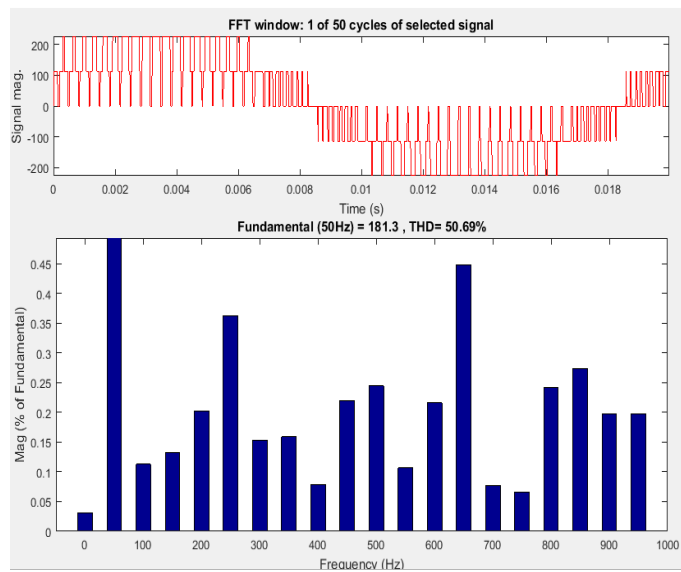
Figure 7. Output and FFT analysis of SPWM inverter.
