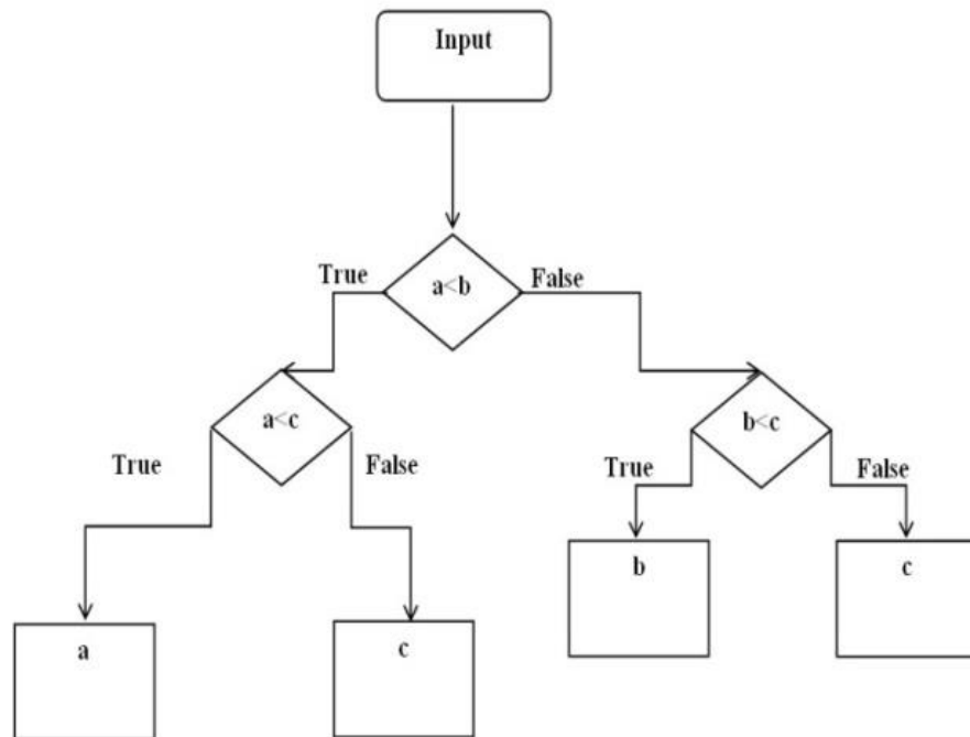
Figure 8: Decision Trees
