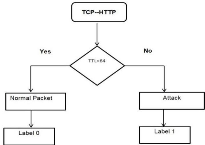
Figure 6: Detecting legitimate and malicious traffic
