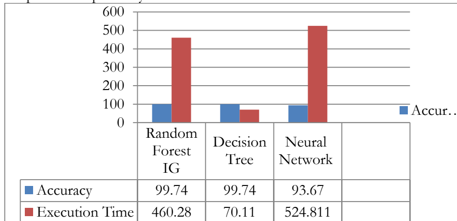
Figure 16: Algorithms Accuracy Comparative Analysis
