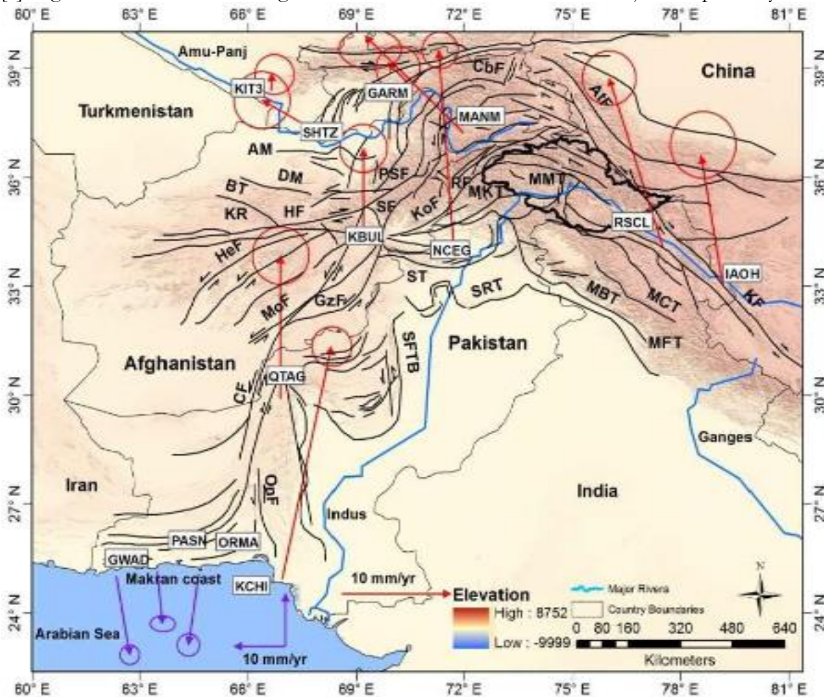
Figure.1 Regional tectonic map showing location of Gilgit Baltistan region
