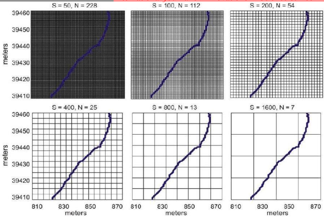
Figure 3. Calculation of Fractal Dimension (FD) by using Box counting method.
