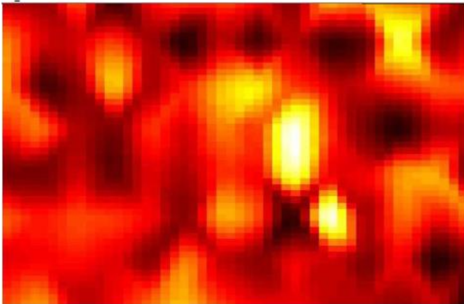
Figure 6: Distribution of map for LA values Low LA values are in black, red are medium and yell
