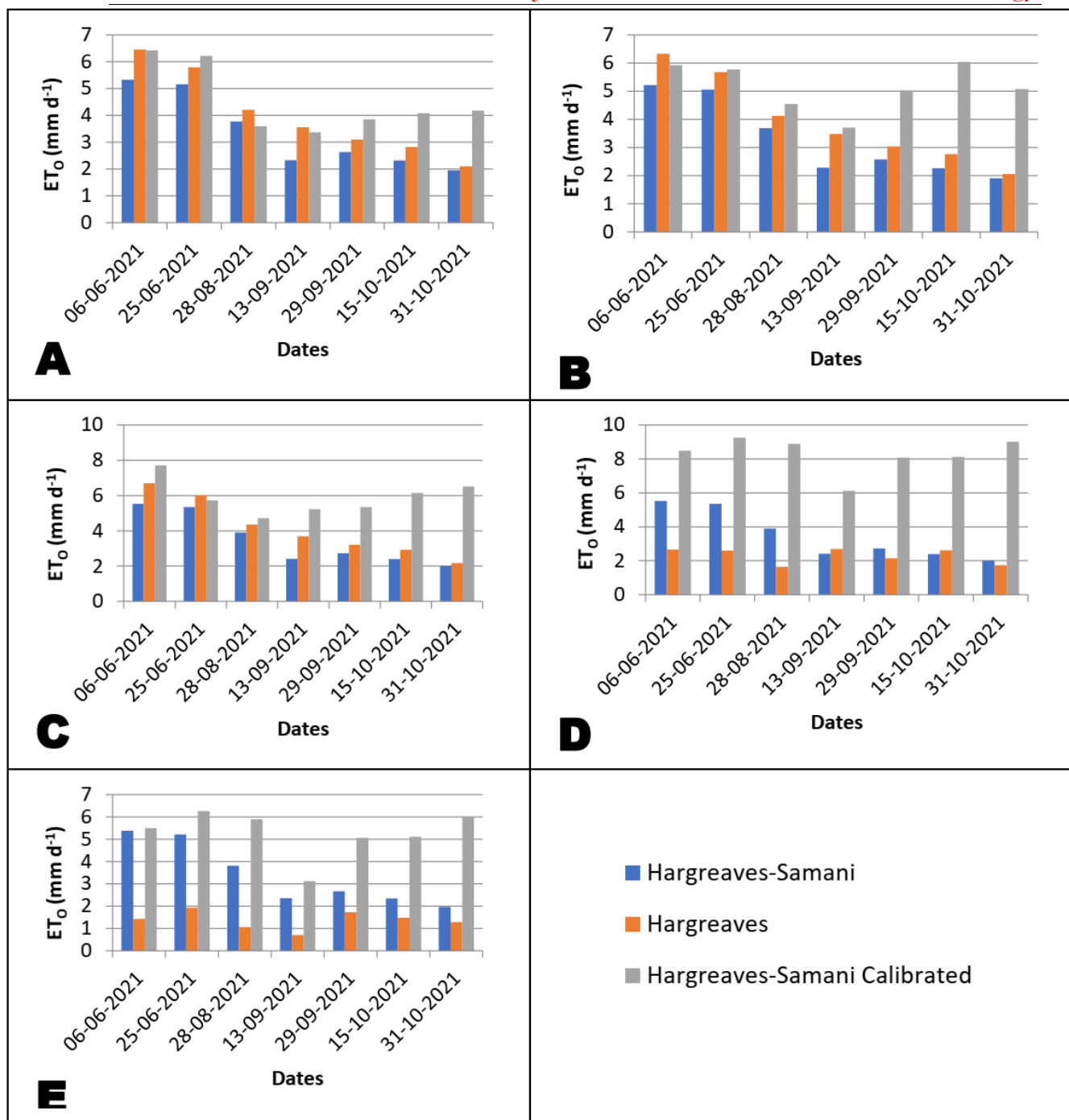
Figure 7: Date wise comparison of ET_0 values estimated through HS, Hargreaves and HS_{CAL} . A) Water B) Trees C) Vegetation D) BuiltUp E) Rangeland
