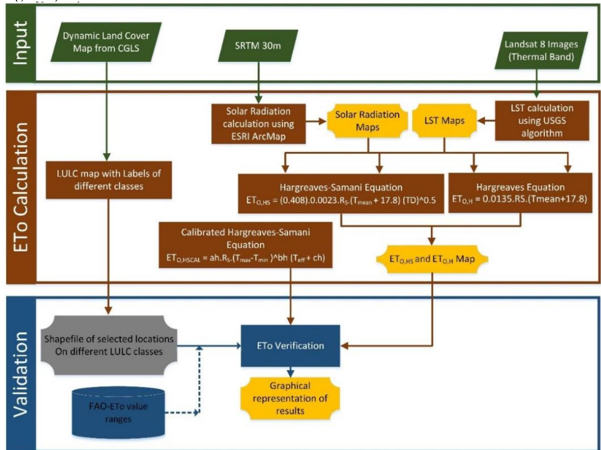
Figure 3: Flow diagram for ET_o retrieval through Hargreaves, Hargreaves-Sammani (HS) and Hargreaves-Sammani Calibrated ( HS_{CAL} ) equations and their verification processes.
