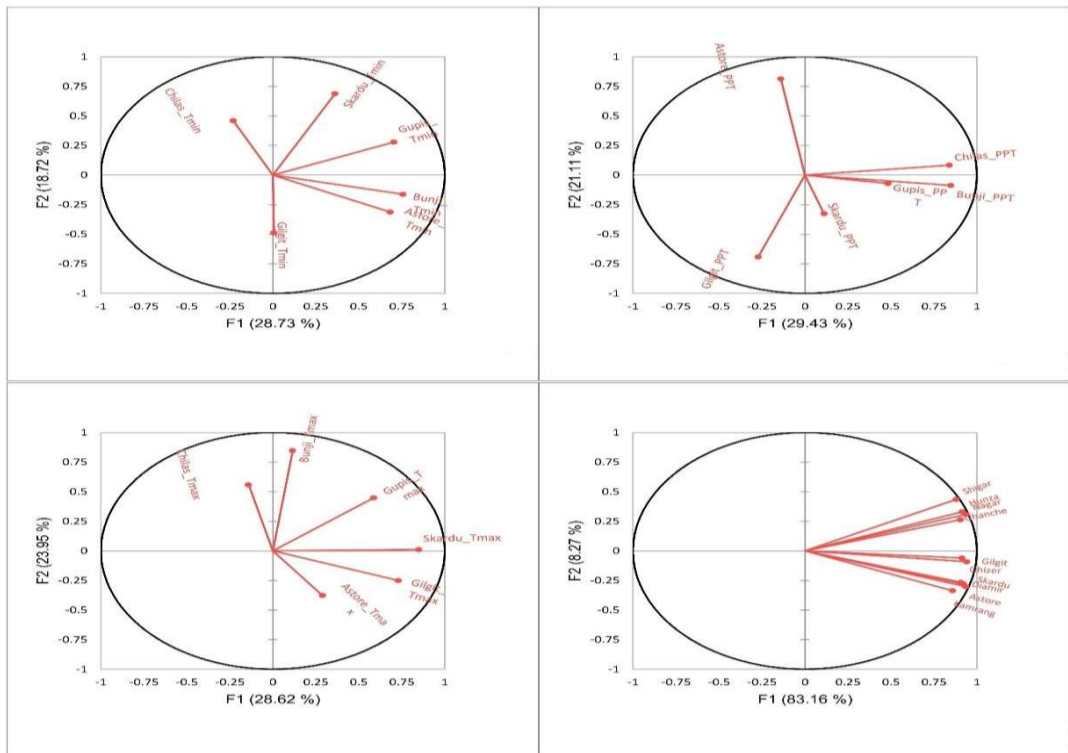
Figure 7. Principal Component Analysis (PCA) for Hydro-meteorological parameters precipitation and minimum temperature, maximum temperature and snow cover of basins Discussion:
