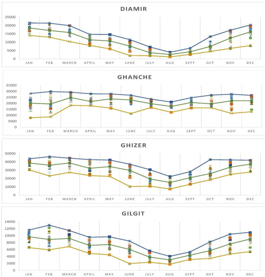
Figure A1: Inter-Annual snow cover inclination and depletion curves from 2000–2020 showing quantitative variations of seasonal snow cover over for Diamir, Gilgit and their sub-basin.
