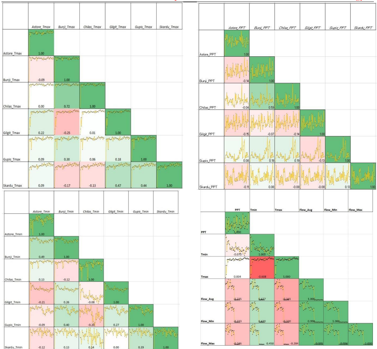
Figure 6. (a) Correlation Matrices Station-wise Maximum Temperature (b) Minimum Temperature (c) precipitation and Flow data at Gilgit Station and runoff at Gilgit river
