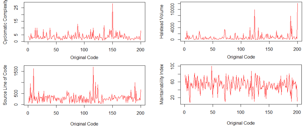
Figure 2. Original Code Results in Line Charts
