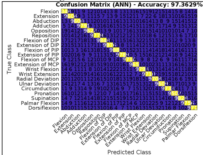
Figure 3. ANN Confusion matrix.
