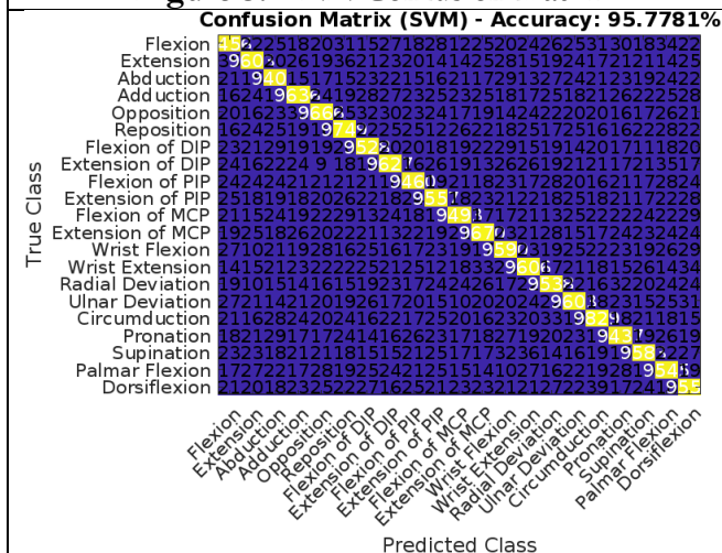
Figure 5. SVM Confusion Matrix
