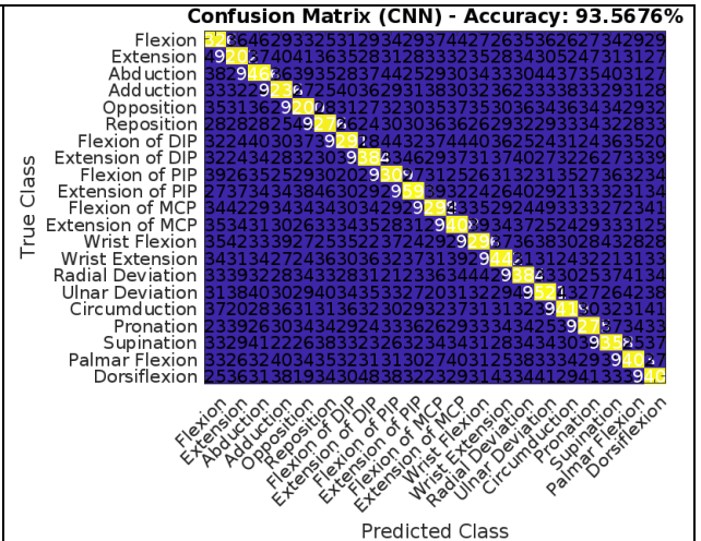
Figure 4. CNN Confusion matrix
