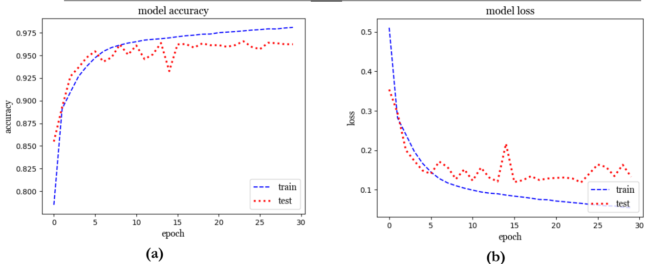
Figure 9. Model Accuracy and Model Loss for Setup-PS-S2cat
