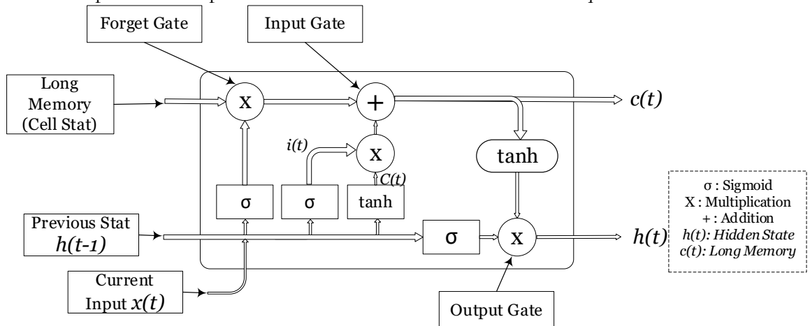
Figure 4. Schematic diagram of LSTM
