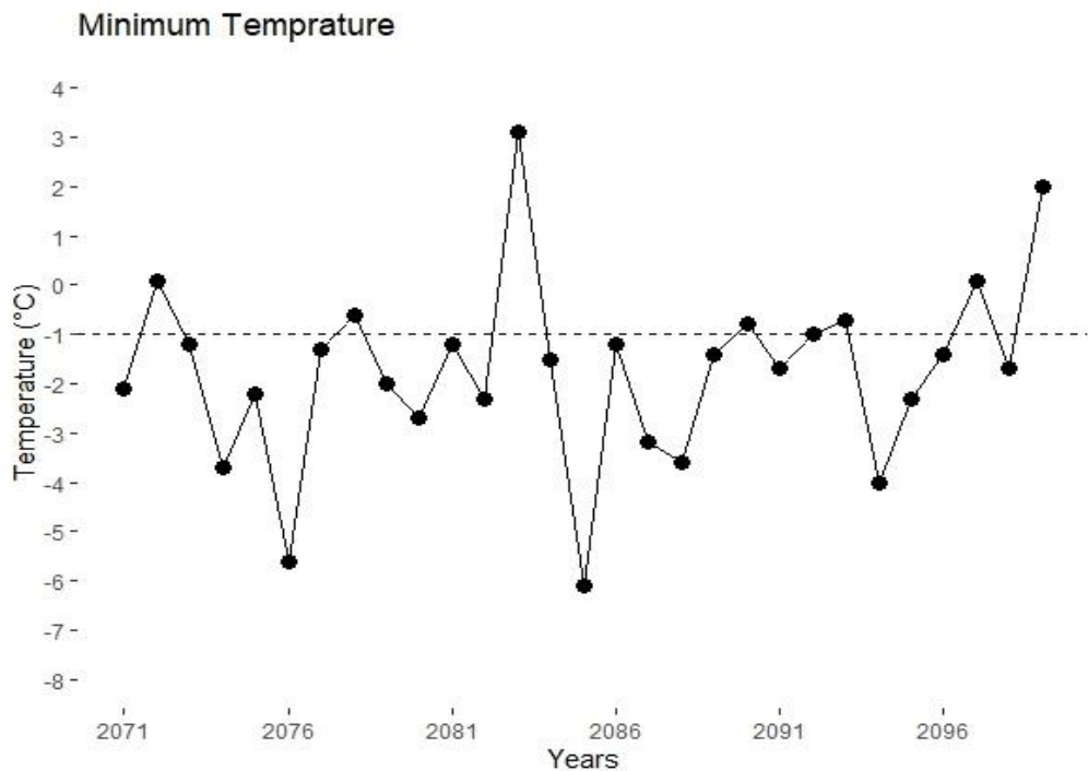
Figure 13 Annual minimum temperature trend for the period of end century (2071-2099).
