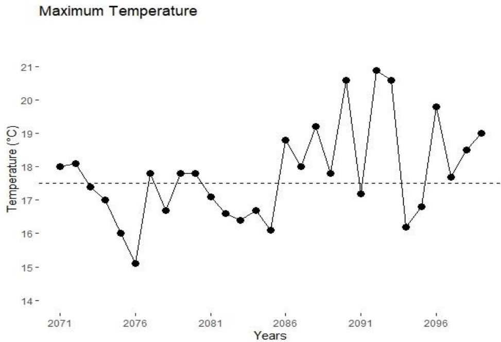
Figure 12 Annual maximum temperature trend for the period of end century (2071-2099)
