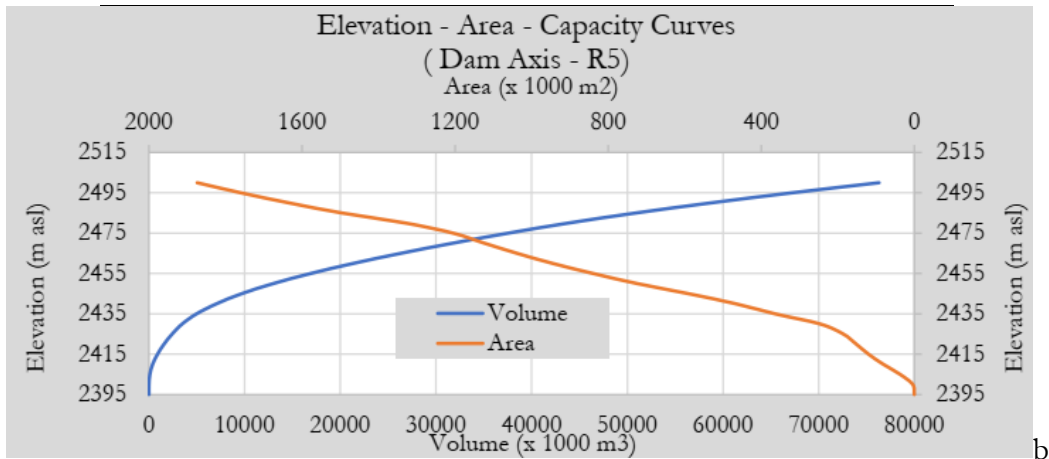
Figure 4. Correlation between elevation, area, and storage capacity for DAM site R5 Comparison of Potential Dam Sites:
