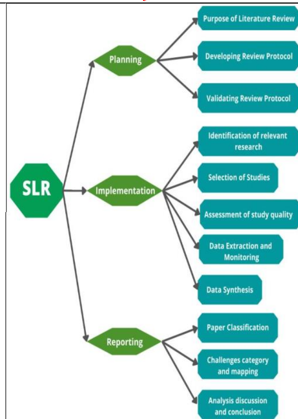
Figure 1: SLR Methodology
