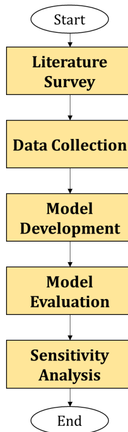
Figure 2: Research Methodology
