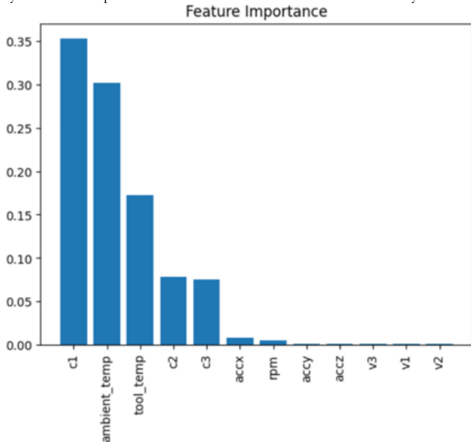
Figure 3: Feature Importance Analysis
