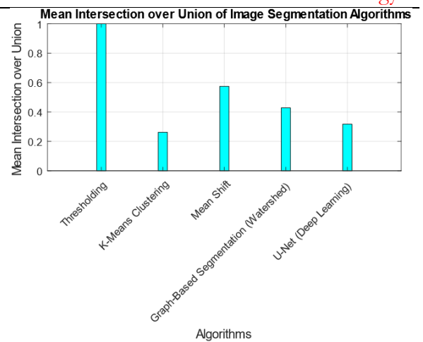
Figure 10: Mean Intersection over Union Comparison Graph
