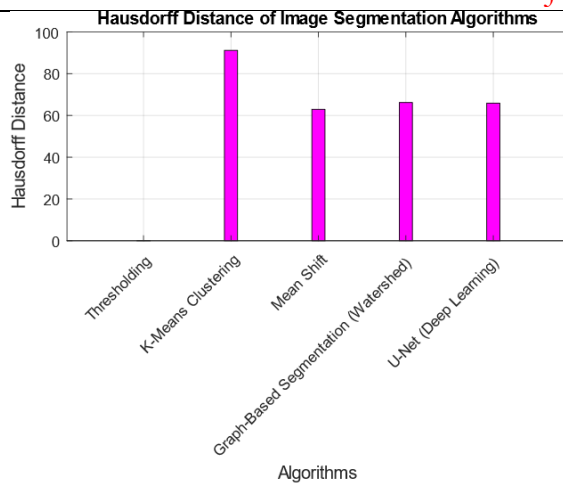
Figure 9: Hausdorff Distance Comparison Graph
