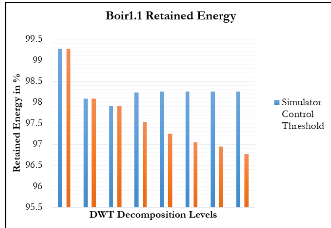
Figure 12: Trend of Bior Splines retained energy.
