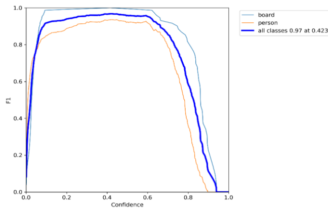
Figure 6. F1 Score for various classes
