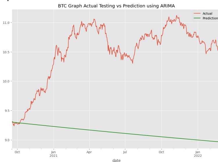
Figure 8: Actual Testing and Prediction using ARIMA Model
