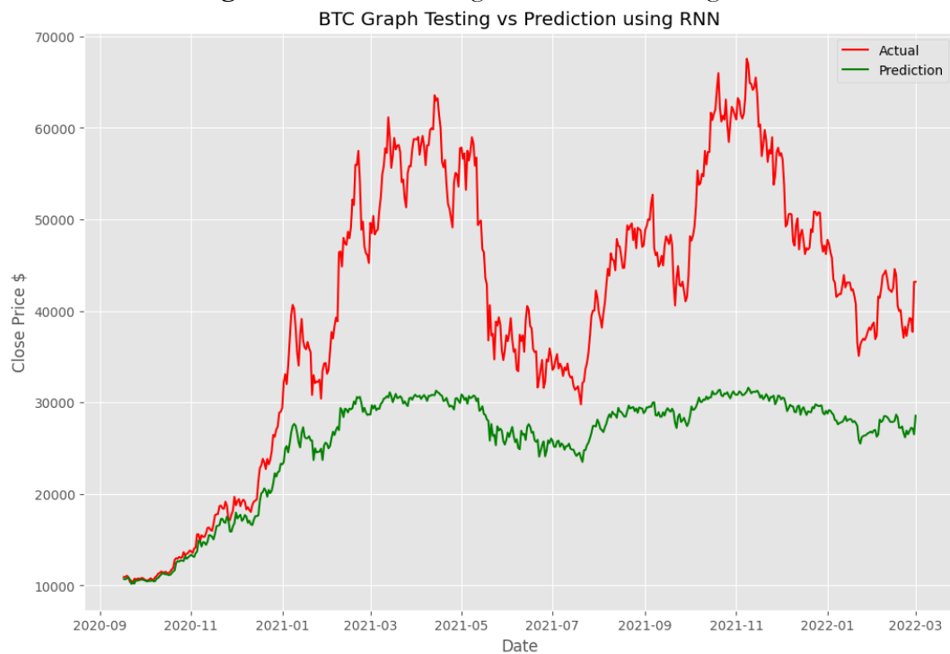
Figure 14: Actual Testing and Prediction using RNN Model
