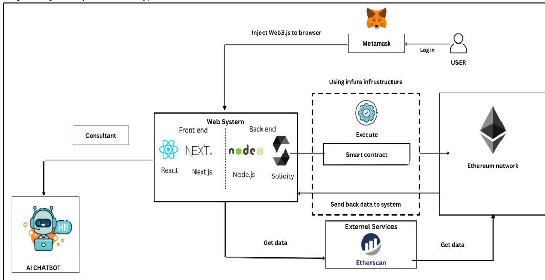
Figure 1: Research Methodology
