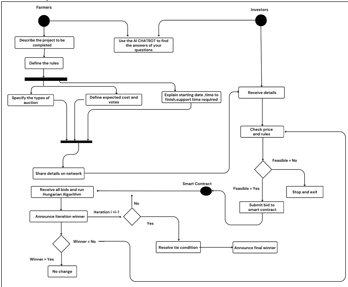
Figure 5: Activity Diagram
