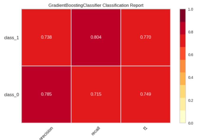
Figure 16: (b) Classification Report of XGBoost Classifier
