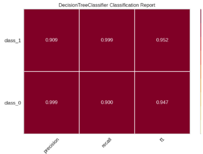
Figure 15: (b) Classification Report of Decision Tree
