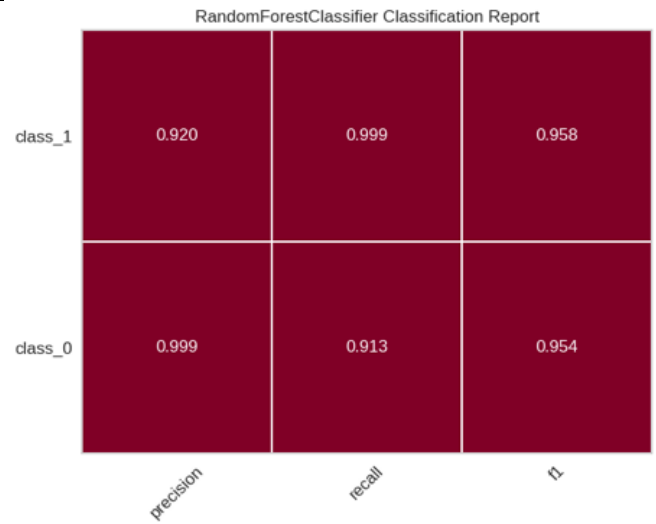
Figure 14: (b) Classification Report of Random Forest
