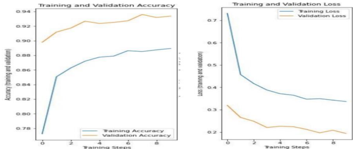
Figure 4: Model training and validation.
