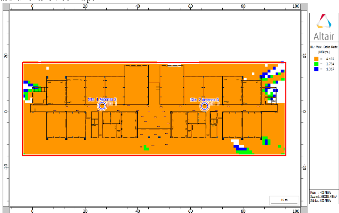
Figure 5: Uplink Data Rate Before Optimization
