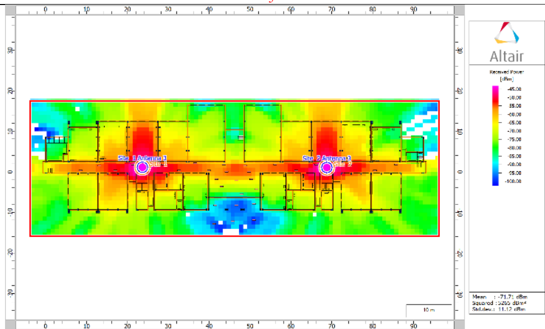
Figure 2: Simulation Values of RSSI After Optimization
