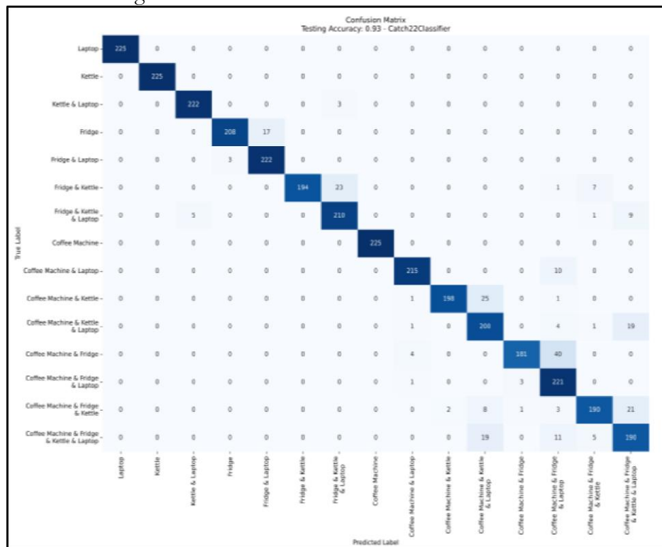
Figure 7: Confusion Matrix for CATCH22 Classifier
