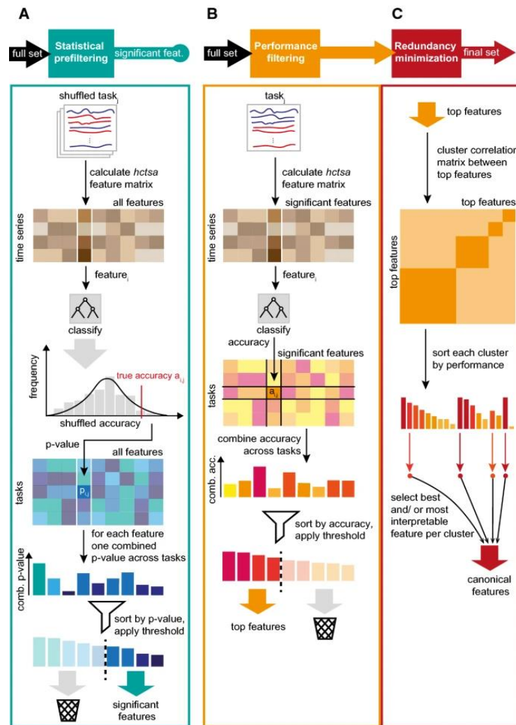
Figure 6: Process of CATCH22 feature selection [22]
