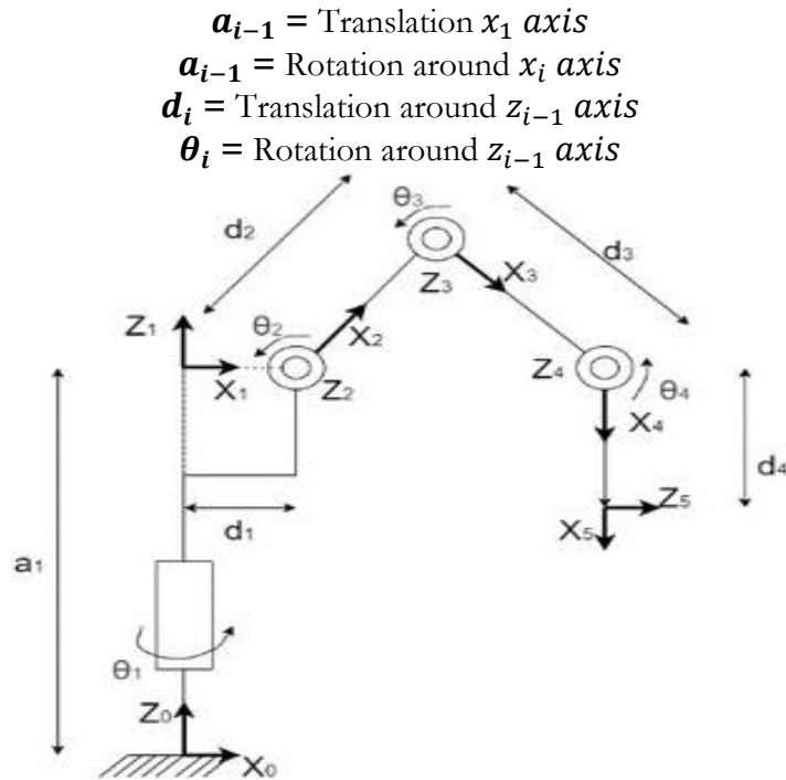
Figure 2: Denavit-Hartenberg Parameters Labeling of 4-Degree-of-Freedom Robot.
