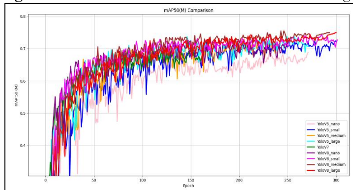
Figure 6: Model training curves of mAP0.5 metric for segmentation masks
