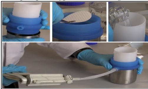
Figure 2: Filtration Assembly Setup, and Method of Using
