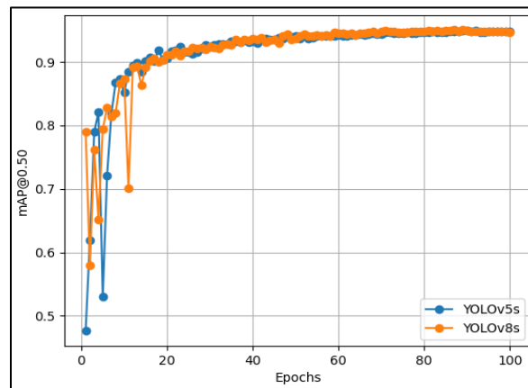
Figure 5: Comparison of YOLOv5s and YOLOv8s on current dataset
