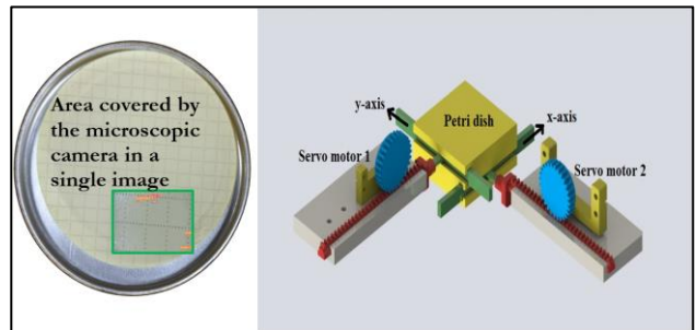
Figure 3: Automatic Moving Petri Dish System Implemented in the Automatic Kit
