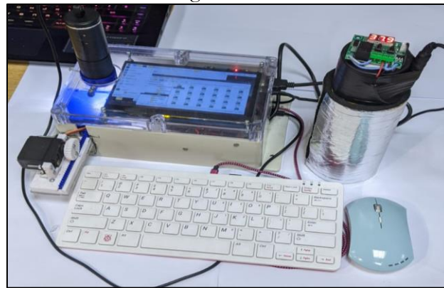
Figure 6: Automatic Imagery System Used for Making Dataset
