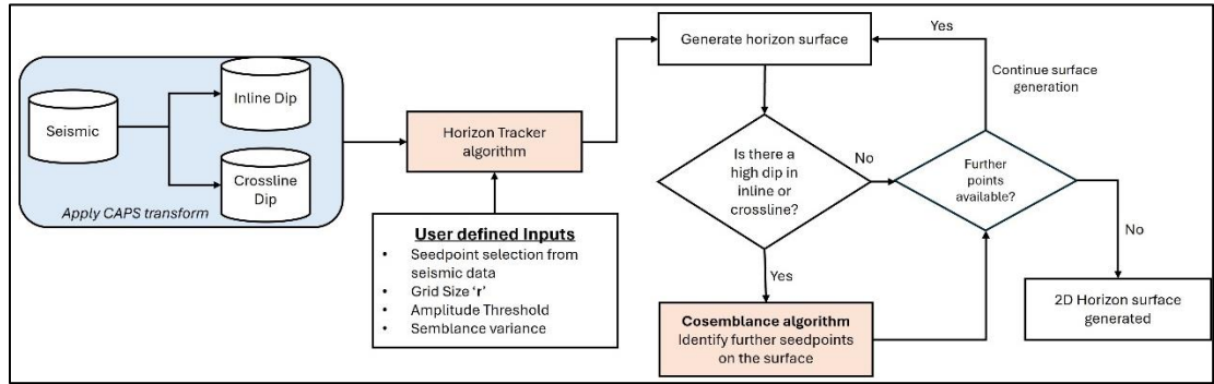
Figure 1: Process of an automated three-dimensional horizon tracker
