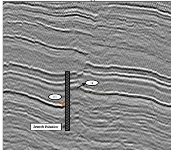
Figure 5: The 3D horizon surface that stopped at seismic data point T1. Spatial grid search was used across the fault using co-semblance algorithm.
