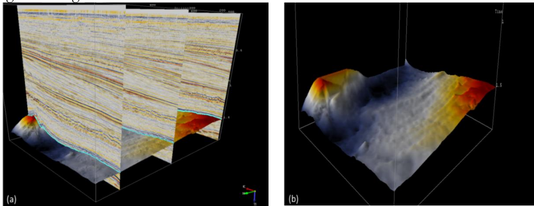
Figure 3: (a) F3 Block Netherlands seismic data along with a tracked horizon surface (b)
