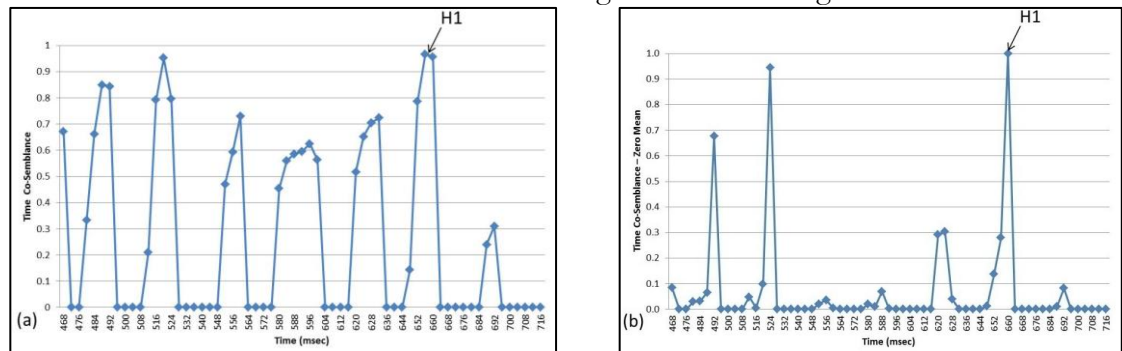
Figure 6: Cossemblance Measurement analysis (a) Time Domain measurements (b) Time Domain measurements with zero mean
