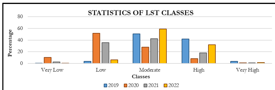
Figure 7: Graph showing statistics of LST classes
