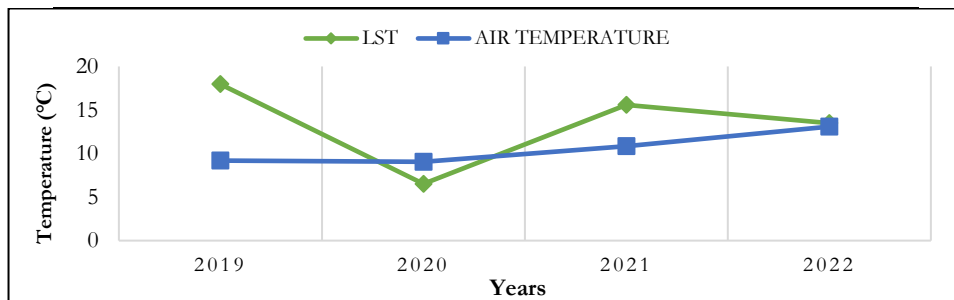
Figure 9: Graph showing the correlation between LST and Air temperature
