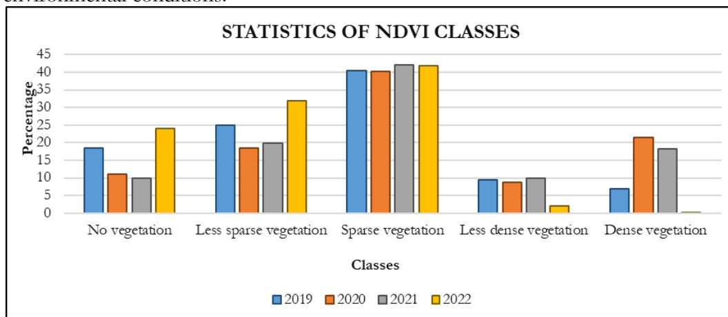
Figure 5: Graph showing statistics of NDVI classes
