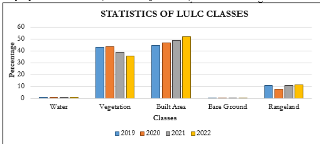
Figure 3: Graph showing statistics of LULC classes
