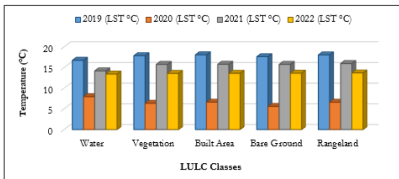
Figure 10: Graph showing LULC Classes with their LST 2019-2022
