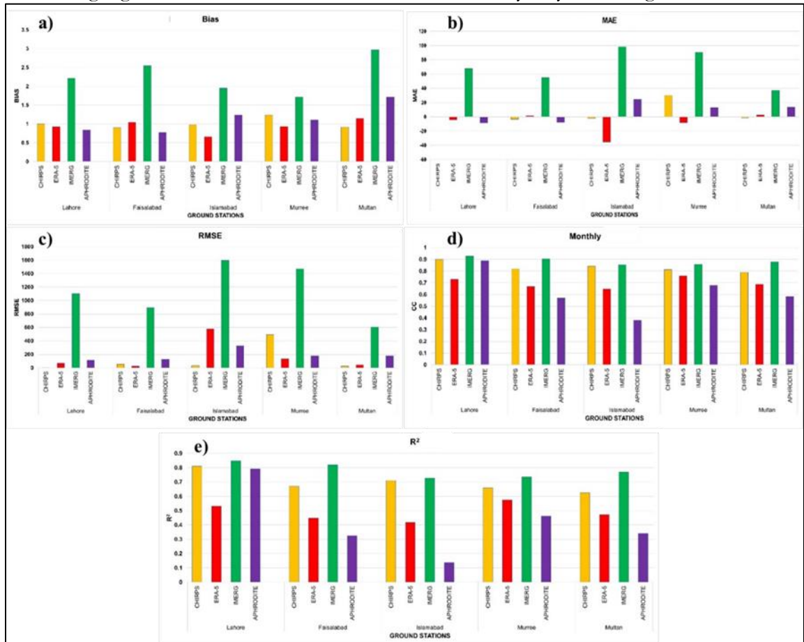
Figure 4: Statistical indicators showing the relationship between the ground station data and daily gridded precipitation datasets at a monthly timescale, a) Bias, b) MAE, c) RMSE, d) CC, and e) R 2 with correspondence observatories from 2001–2022.
