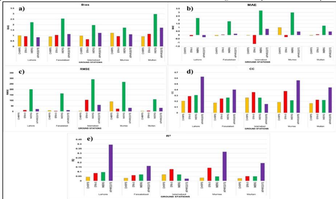
Figure 3: Statistical indicators showing the relationship between the ground station data and daily gridded precipitation datasets a) Bias, b) MAE, c) RMSE, d) CC, and e) R2 with correspondence observatories from 2001–2022.
