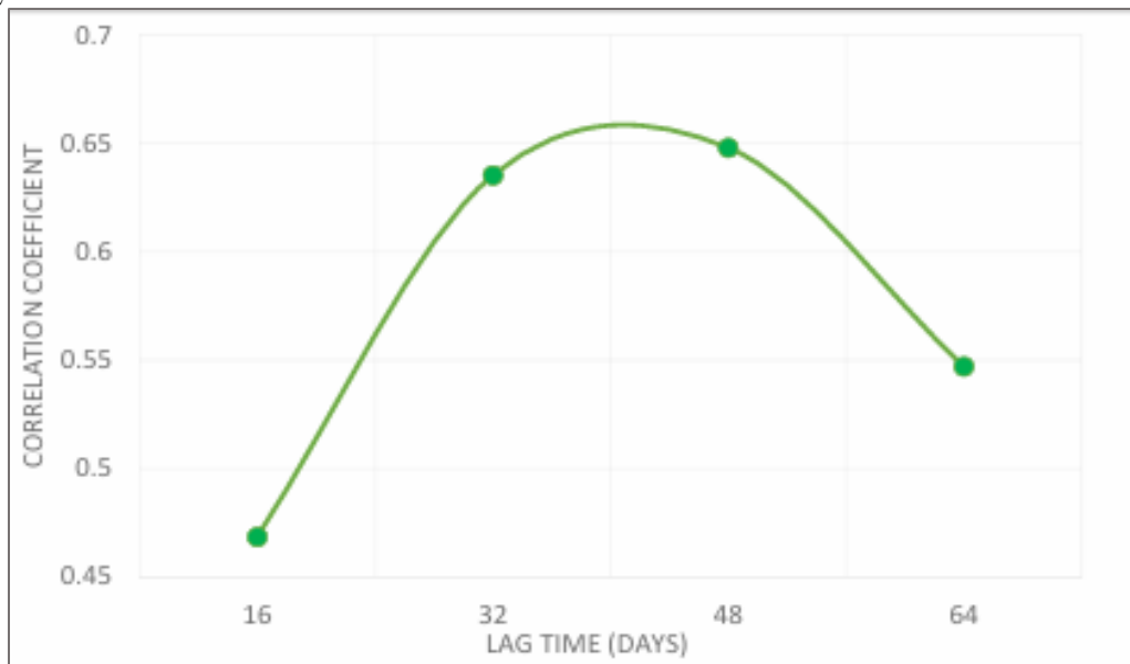
Figure 4: Fix lag window correlation between NDVI and Precipitation
