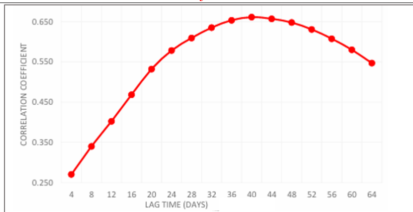
Figure 5: Fix lag window correlation between NDVI and Precipitation
