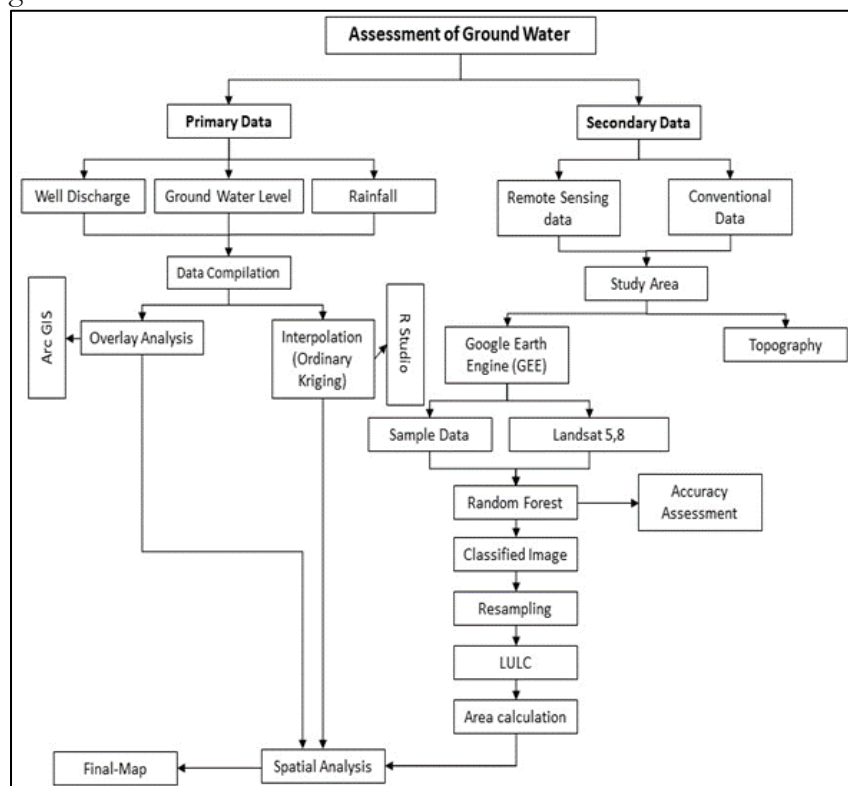
Figure 2: Flow Chart Visualizing the Data Processing and analysis Methodology
