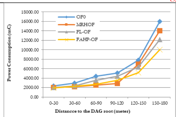
Figure 8 (b). Power Consumption in Random Topology
