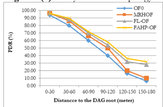
Figure 7 (b). PDR in Random topology
