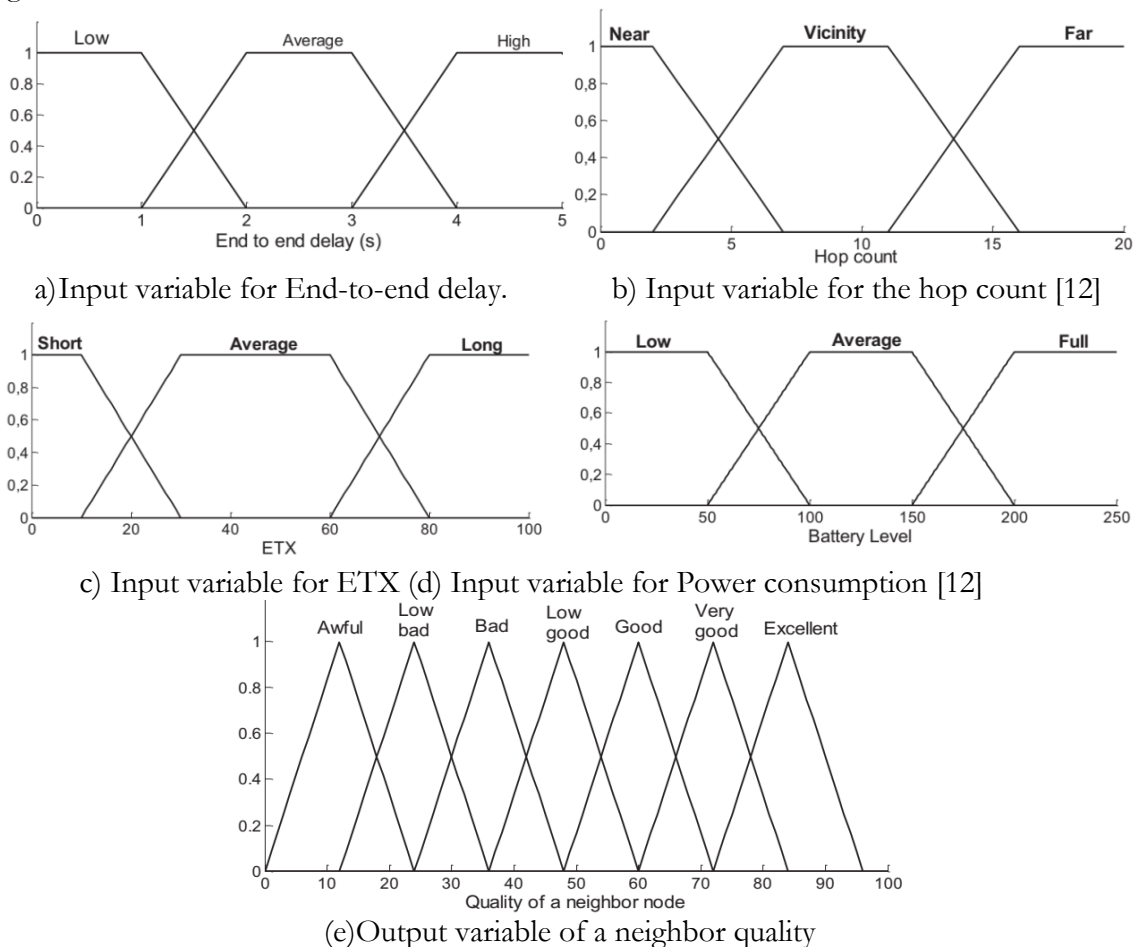
Figure 3. Definition of membership functions [12]
