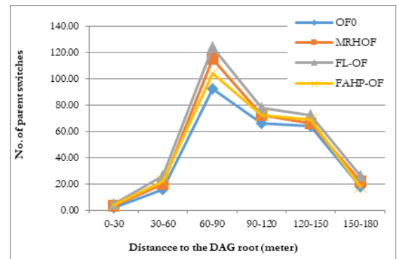
Figure 9 (b). Parent switching in Random topology
