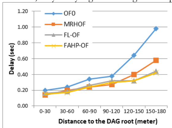
Figure 6 (a). Delay in grid topology
