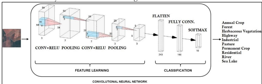
Figure 6: An Example of a Convolutional Neural Network.
