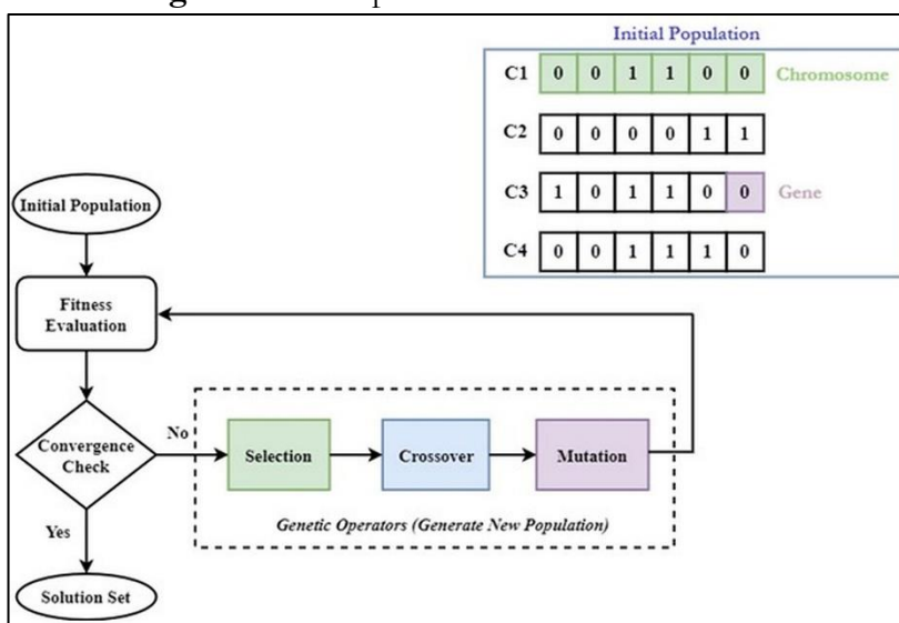
Figure 3. Flow Chart of Genetic Algorithm with Sample Initial Population.
