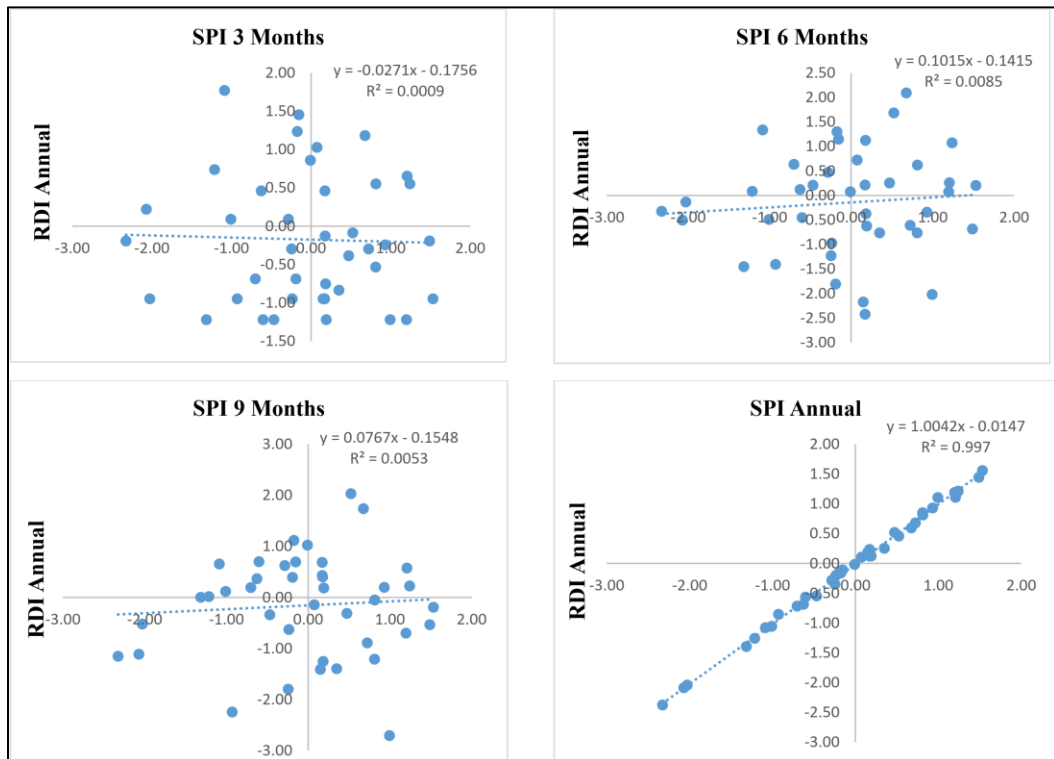
Figure 5: Comparison of SPI 3-, 6-, 9- and 12-months Vs. RDI Annual (Mirpurkhas)
