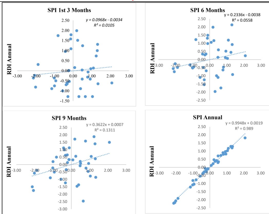
Figure 8: Comparison of SPI 3-, 6-, 9- and 12-months Vs. RDI Annual (Umerkot)
