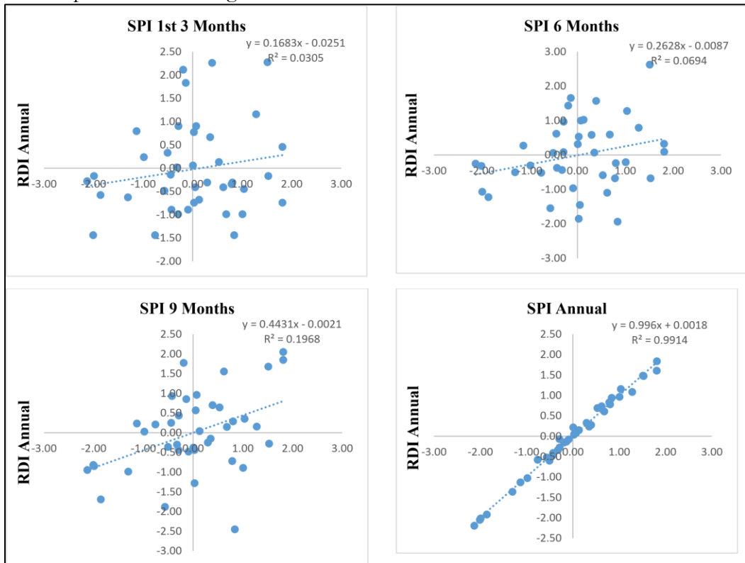
Figure 6: Comparison of SPI 3-, 6-, 9- and 12-months Vs. RDI Annual (Shanghar)
