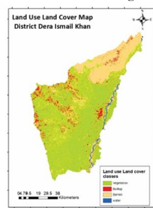
Figure 2: Land use Land cover of D.I Khan
