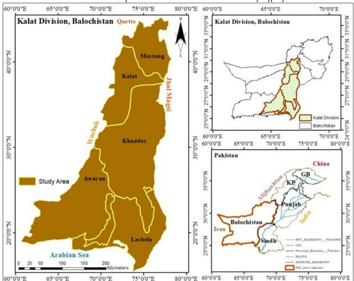
Figure 1: Study Area Map Kalat Division, Balochistan
