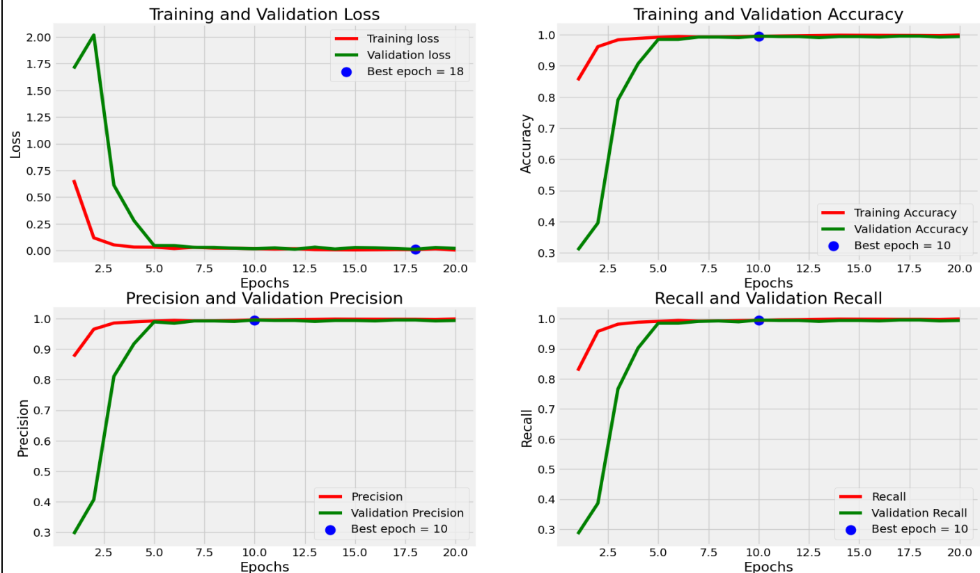
Figure 5: Shows the Performance of the Proposed Model.
