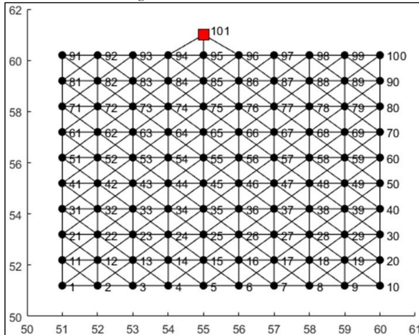
Figure 2: Arrangement of nodes in a grid topology.
