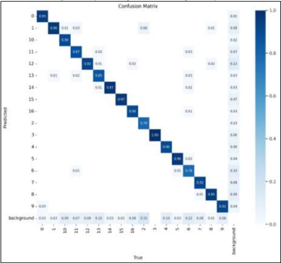
Figure 7. Confusion matrix.
