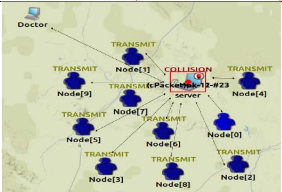
Figure 2. OMNet++ discrete event simulator to be used in WBAN [13]
