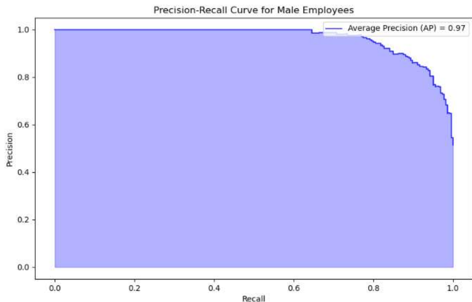
Figure 10 Precision-Recall Curve for Male Employee Data
