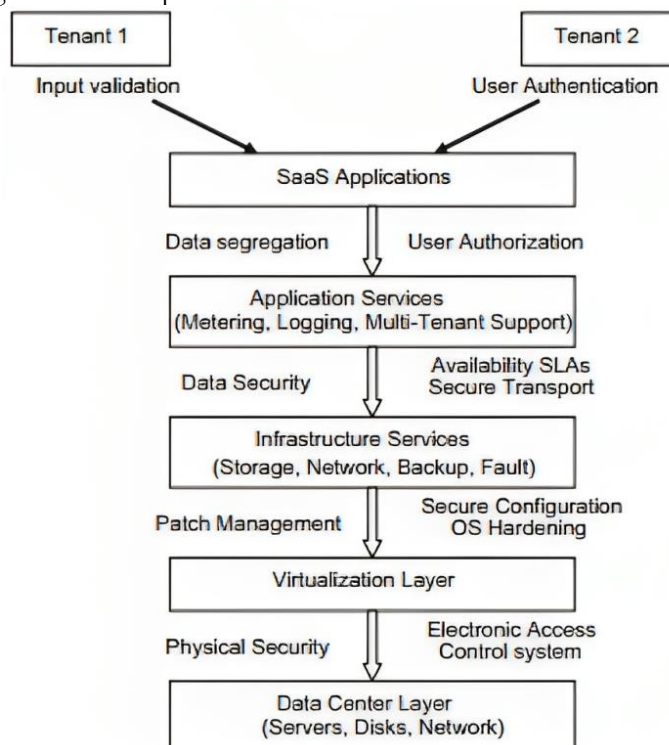
Figure 3. SaaS Security
